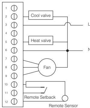
Typical wiring for ON/OFF control in 4 pipe 1H/1C Auto/Manual Change over (VC4013)
