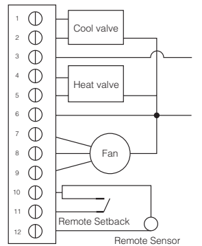
Typical wiring for 3-wire control in 4 pipe 1H/1C Auto/Manual Change over (VC6013)
